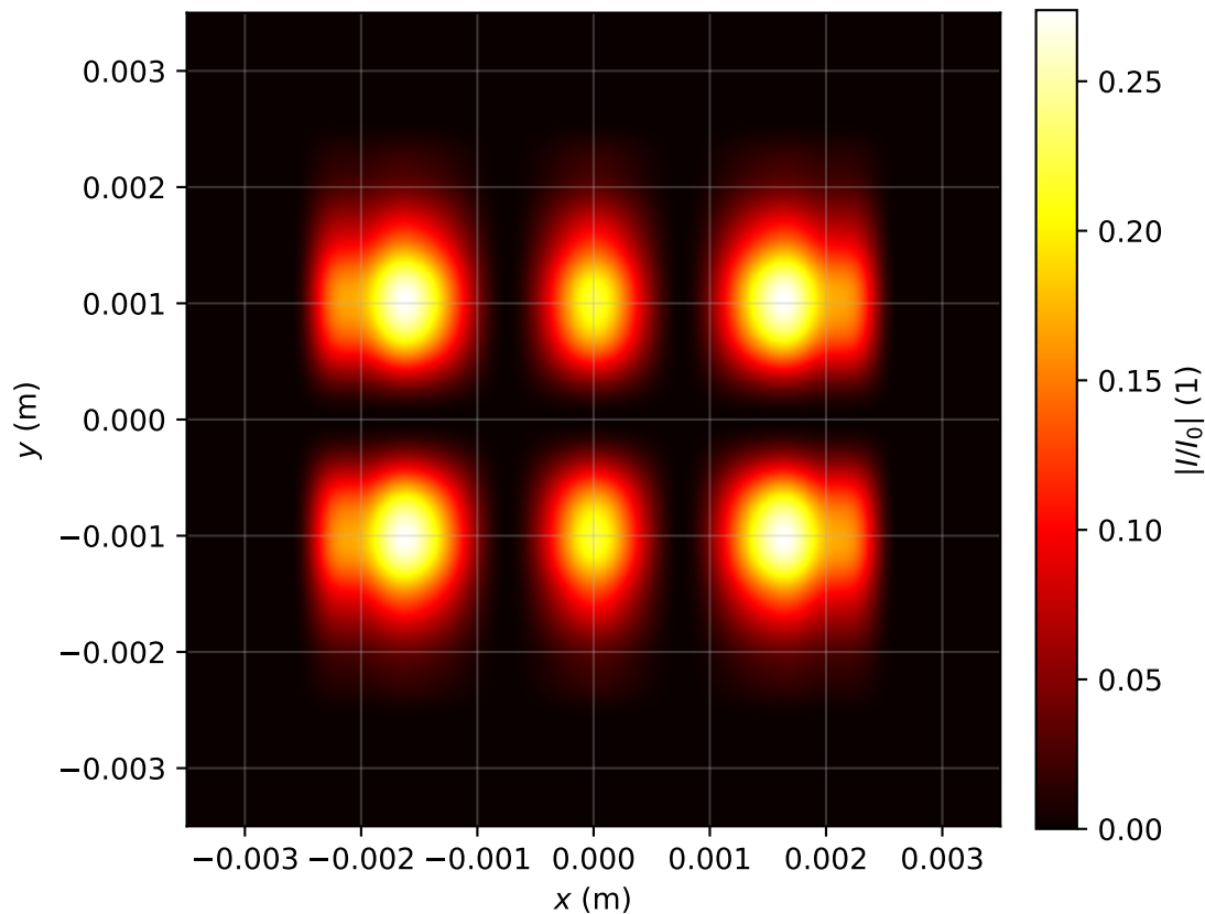
Intensity profile I(x, y, z = 3.662)/I_0 , P_{in}=1.0P_{cr} , artificial time
